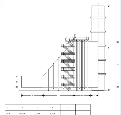
SITE AND COMPONENT LAYOUT
