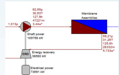
GTCC + SEAWATER DESALINATION
